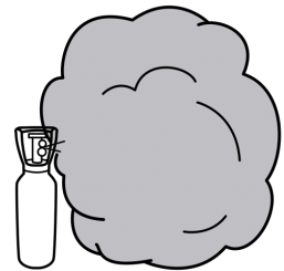
Xenon
